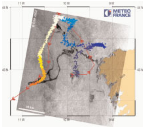
FIGURE 1 (A) : DRIFT WITH MERCATOR CURRENT AT 3 M
