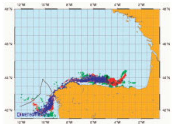
FIGURE 4: 13 DECEMBER 2002 AT 12 UTC. COMPARISON BETWEEN MODELS AND IN SITU OBSERVATION BASED ON A CONSTANT LEAKAGE ALONG THE TANKER'S TRAJECTORY (SHOWN IN BLACK). MOTHY IS IN BLUE. MOTHY+MERCATOR IN GREEN AND MOTHY+FOAM IN RED. BLACK TRIANGLES ARE THE OBSERVED SLICKS.
