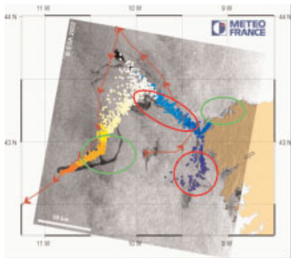
FIGURE 1 (B) : DRIFT WITH OPERATIONAL MODEL MOTHY
